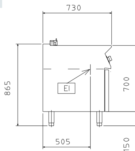
Side
